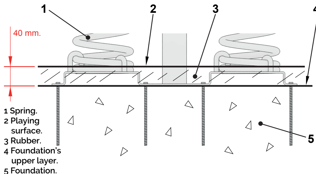
Spring Anchoring detail.
