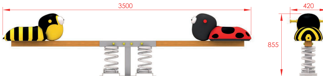
General dimensions (in millimeters)
