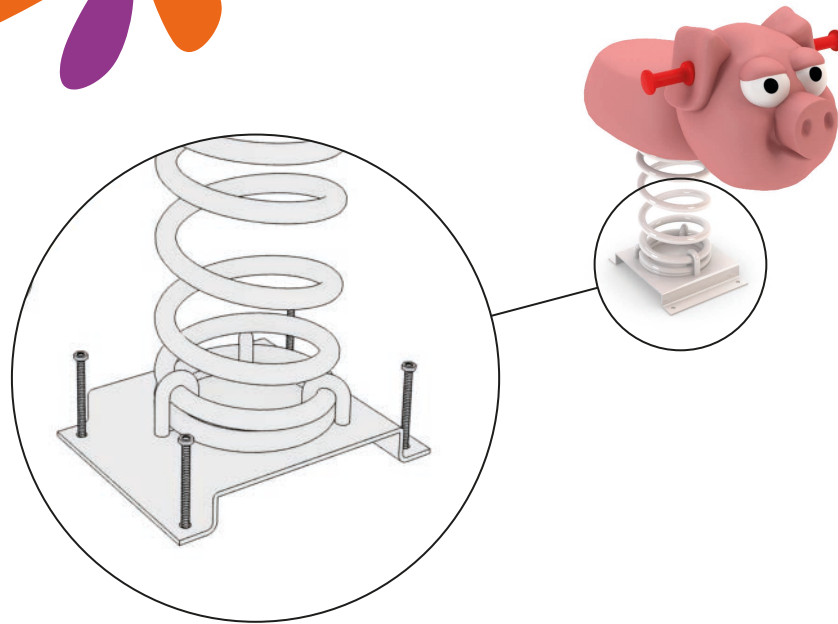
Anchoring detail
