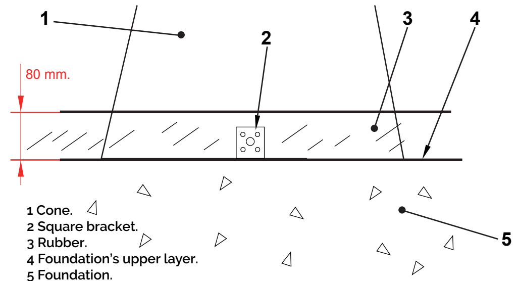
Anchoring detail
