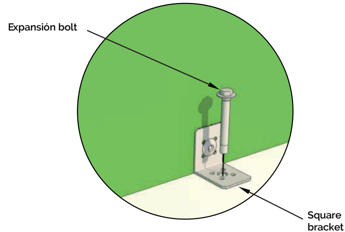
Anchoring detail.
