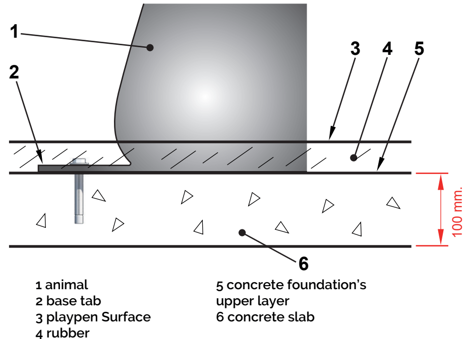
Anchoring details
