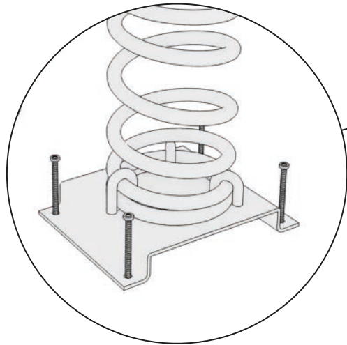
Anchoring detail
