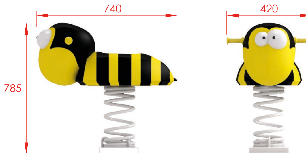
General dimensions (in millimeters)
